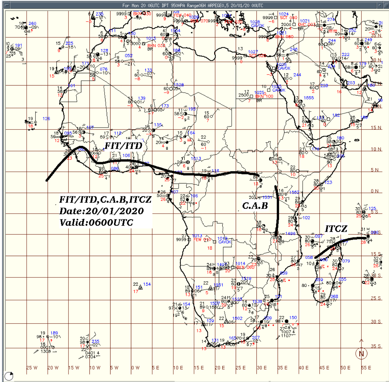
Tabulated positions of the ITD: 20 th JANUARY 2020
